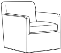
Madelaine / 4452-05SW Swivel Chair (28.5W) Outside: 28.5W x 34D x 33H Inside: 21W x 21D
