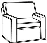
CD87 Series / CD8705T-SW Swivel Chair (34W) Outside: 34W x 38D x 38H Inside: 22W x 22D
